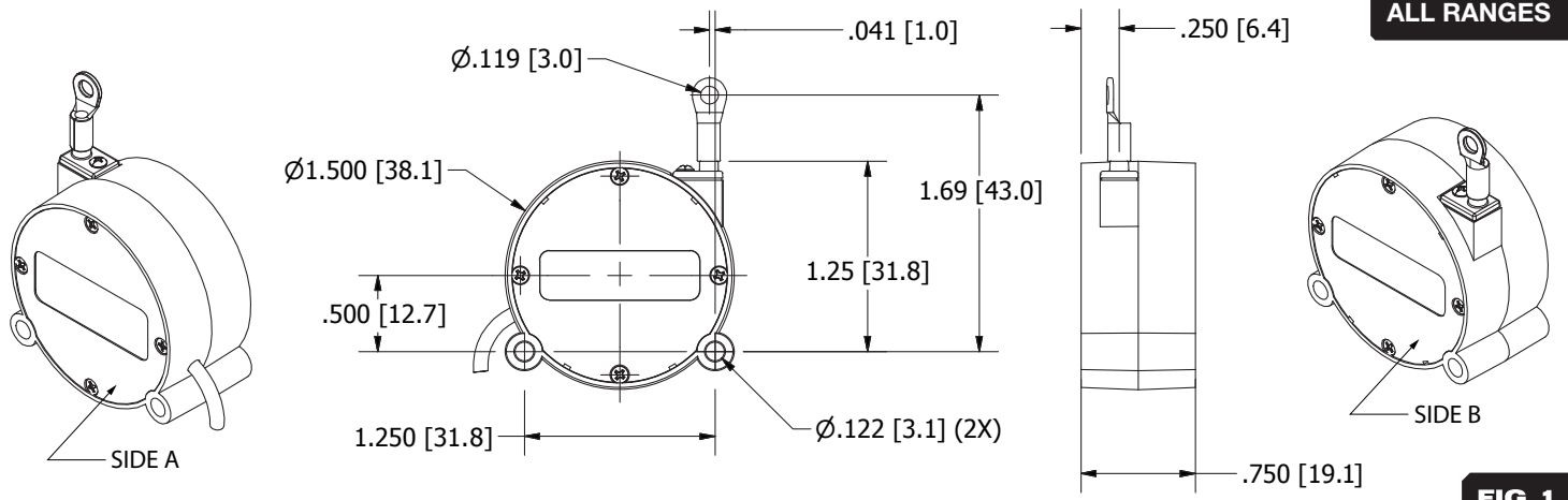
Dimensions in brackets are millimeters.
