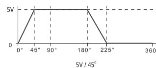
OUTPUT SIGNAL
