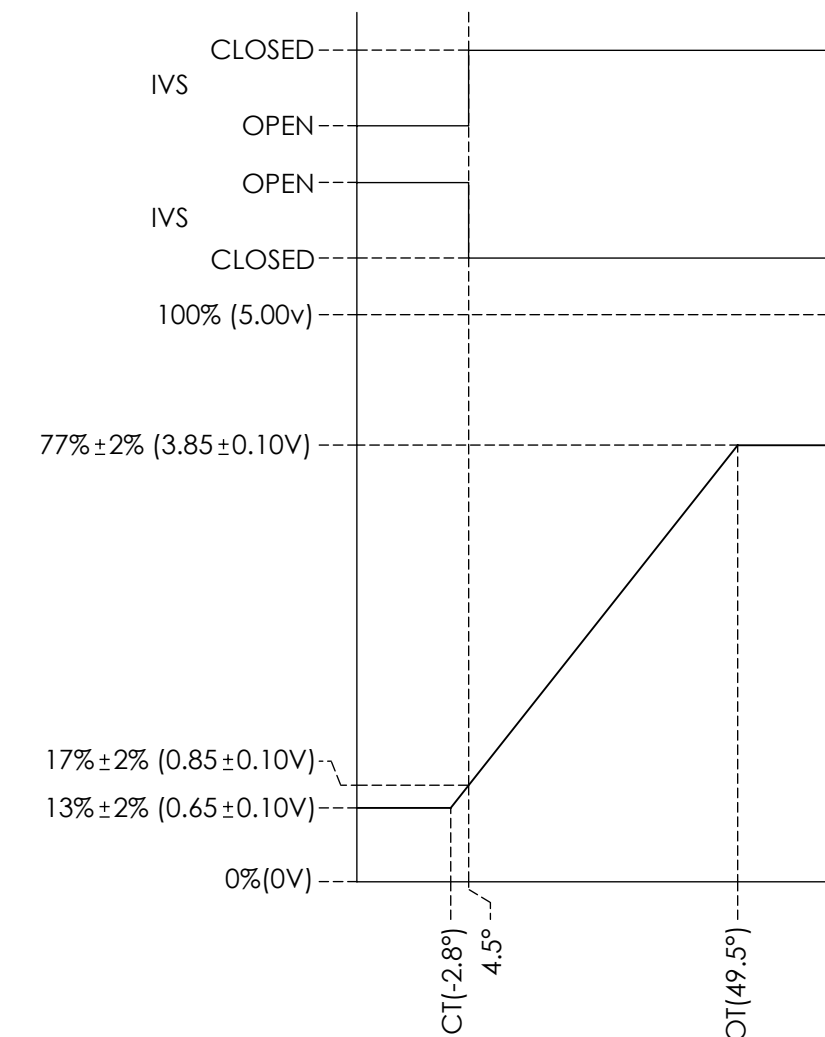
SENSOR ELECTRICAL OUTPUT FIGURE 1
